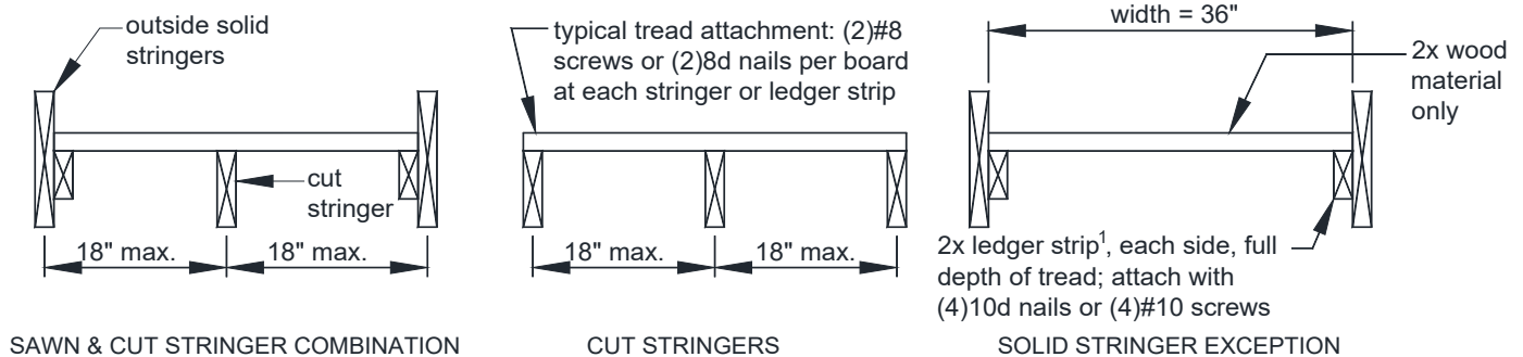
FIGURE 42: STRINGER TREADS
