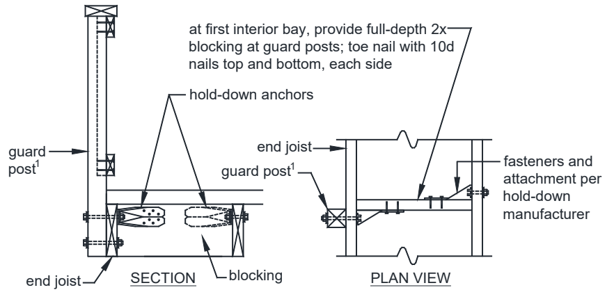
FIGURE 37: GUARD POST-TO-END JOIST
