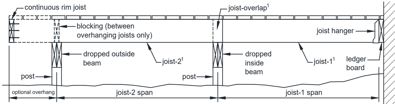
FIGURE 7: MULTI-SPAN DECK - JOISTS WITH DROPPED BEAMS
