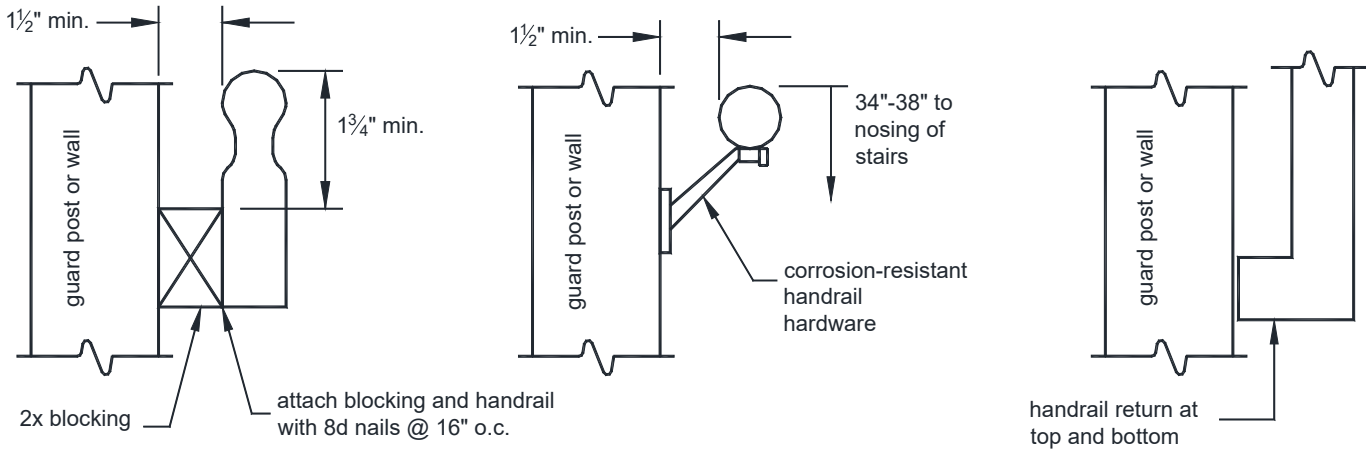
FIGURE 44: HANDRAILS
