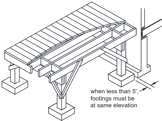
FIGURE 16: FOOTINGS ADJACENT EXISTING HOUSE
