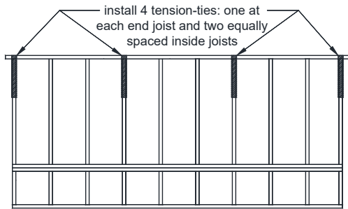
FIGURE 28: METHOD 1 – TENSION TIE LOCATIONS
