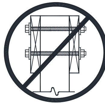
FIGURE 20: PROHIBITED CONNECTION
