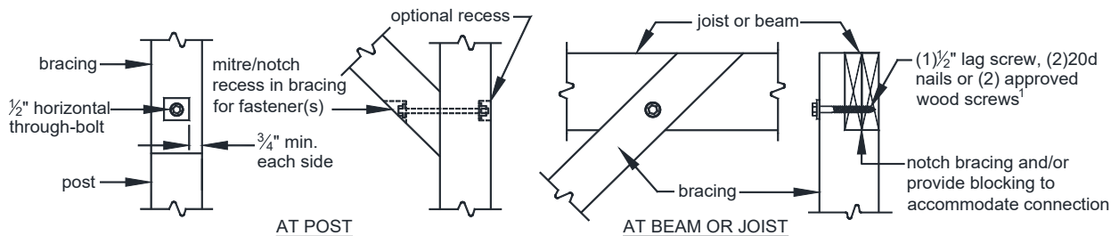
FIGURE 33: TYPICAL CONNECTIONS OF 6x6 KNEE-BRACING
