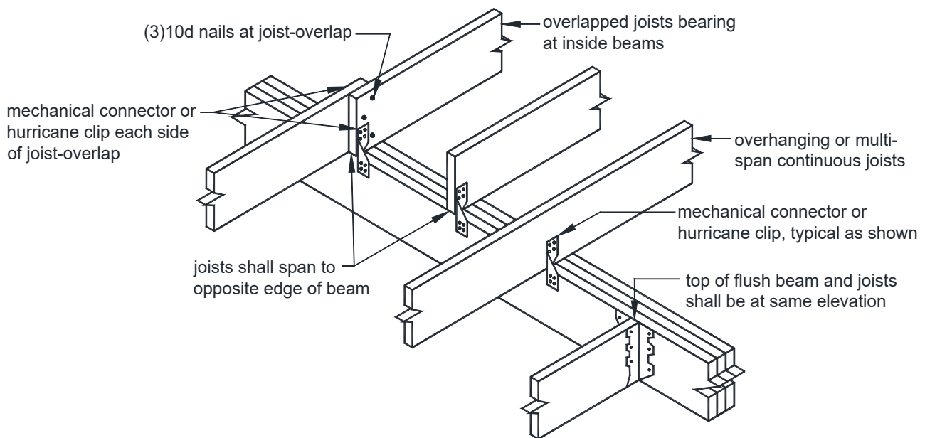
FIGURE 12: JOIST-TO-BEAM CONNECTION
