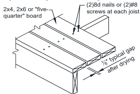
FIGURE 1: TYPICAL DECKING
