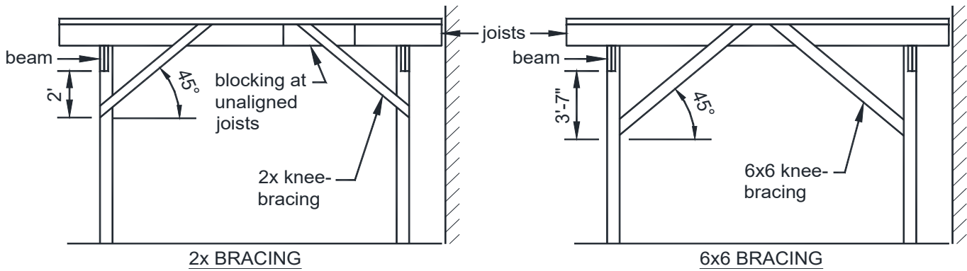
FIGURE 13: METHOD 3 - KNEE-BRACING AT JOIST-POST LOCATIONS
