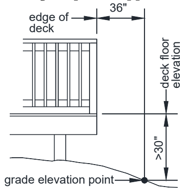
FIGURE 34: WHEN A GUARD IS REQUIRED
