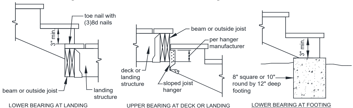
FIGURE 40: STRINGER BEARING
