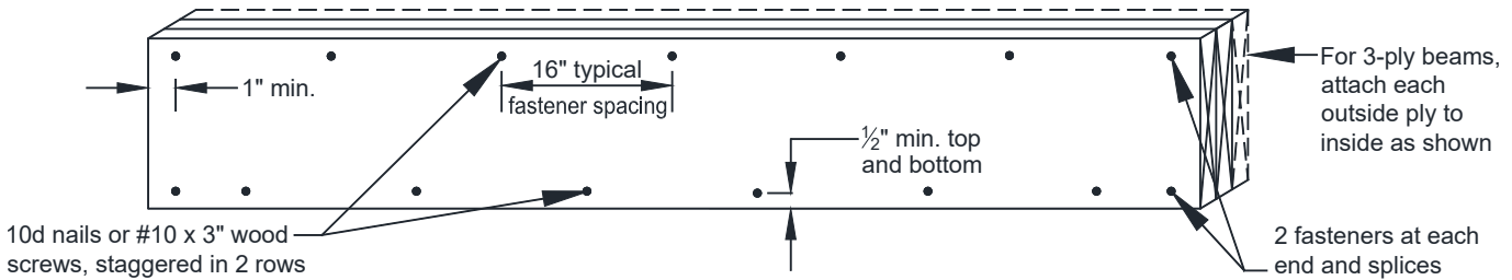
FIGURE 15: BEAM PLY FASTENING
