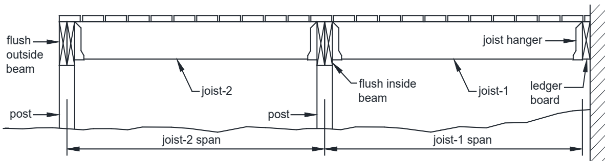
FIGURE 8: MULTI-SPAN DECK - JOISTS WITH FLUSH BEAMS
