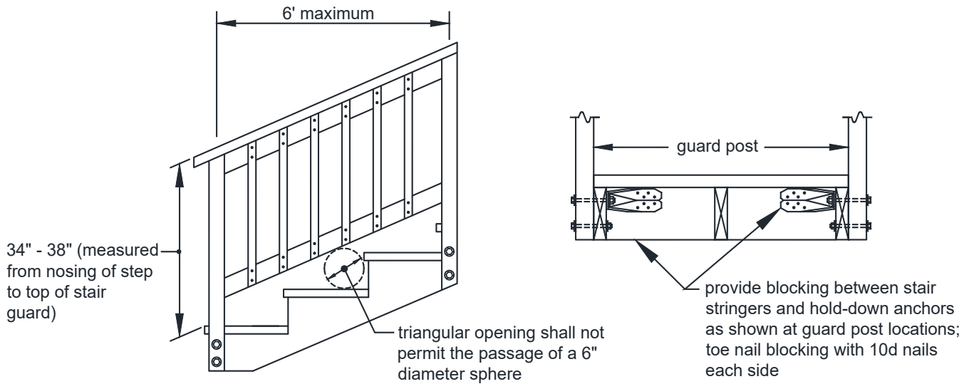
FIGURE 43: STAIR GUARD
