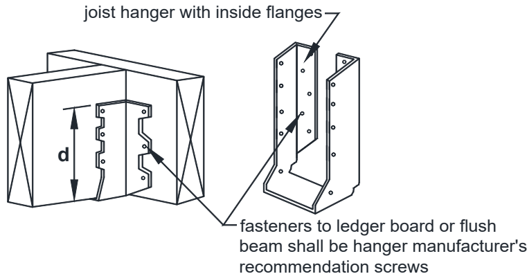
FIGURE 11: JOIST HANGERS
