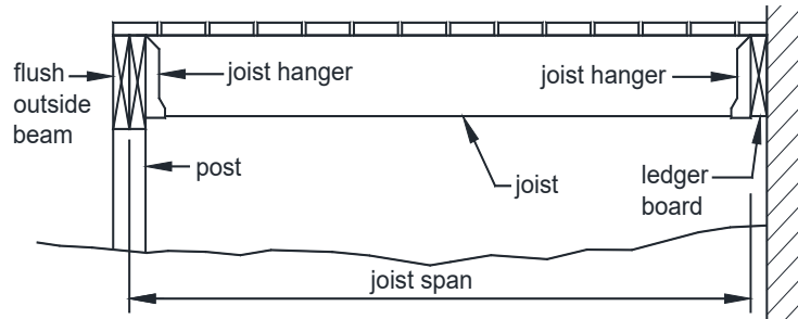
FIGURE 6: SINGLE SPAN DECK - JOISTS ATTACHED AT HOUSE WITH FLUSH BEAM
