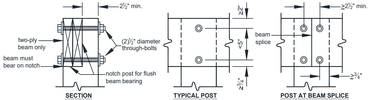
FIGURE 18: NOTCHED 6x6 POST-TO-BEAM CONNECTION
