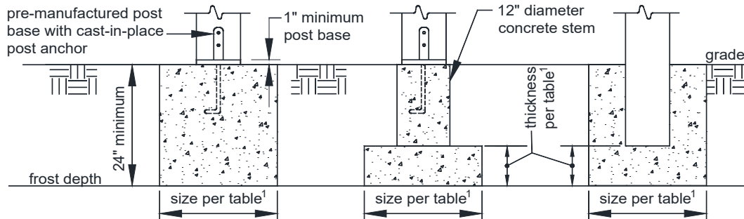
FIGURE 17: FOOTINGS
