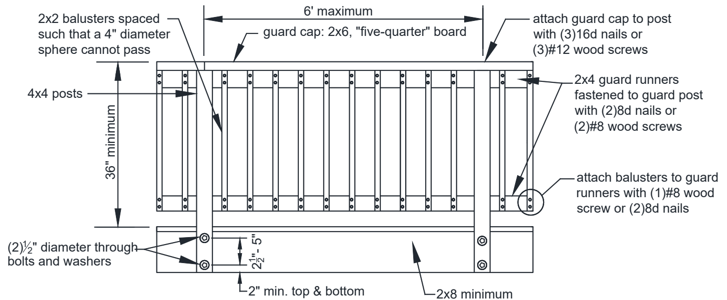
FIGURE 35: GUARD CONSTRUCTION
