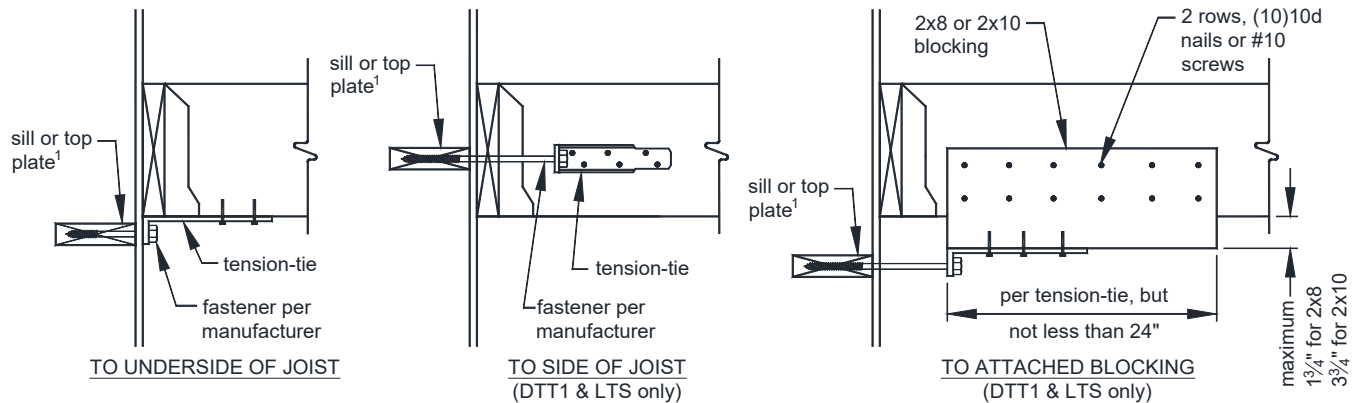
FIGURE 28: METHOD 1 – TENSION TIE LOCATIONS
