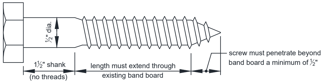
FIGURE 27: LAG SCREW
