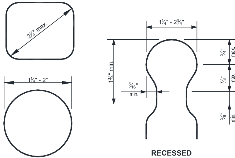
FIGURE 45: HANDRAIL GRASPABILITY
