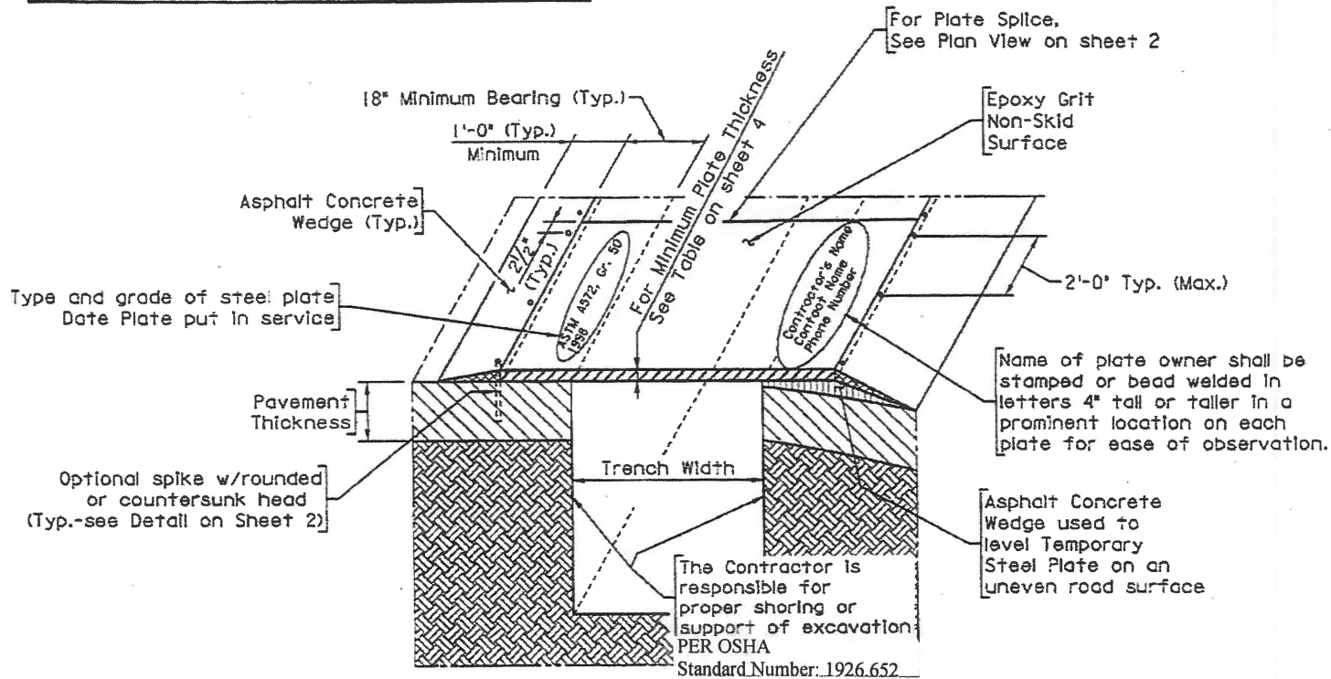
TYPICAL SECTION - TEMPORARY STEEL PLATE BRIDGING Roadway Speed Limit 35 mph or less
