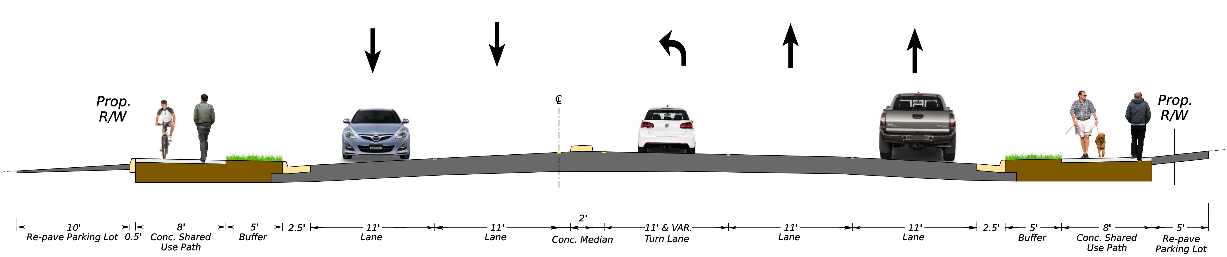
PROPOSED TYPICAL SECTION B-B
