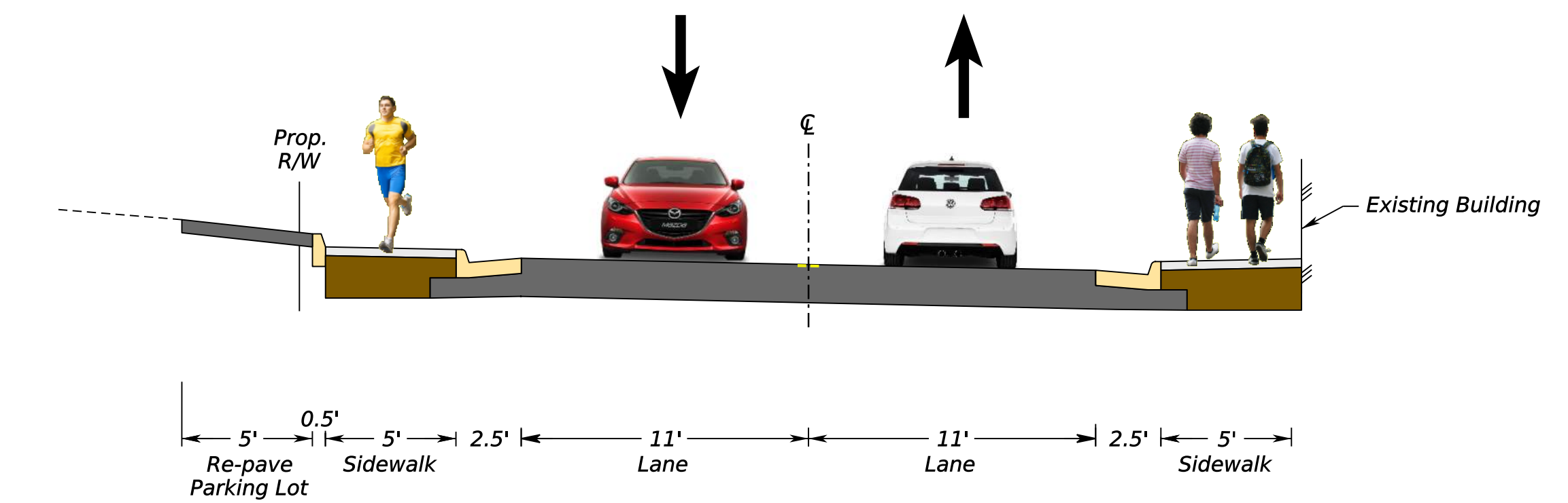
PROPOSED TYPICAL SECTION D-D
