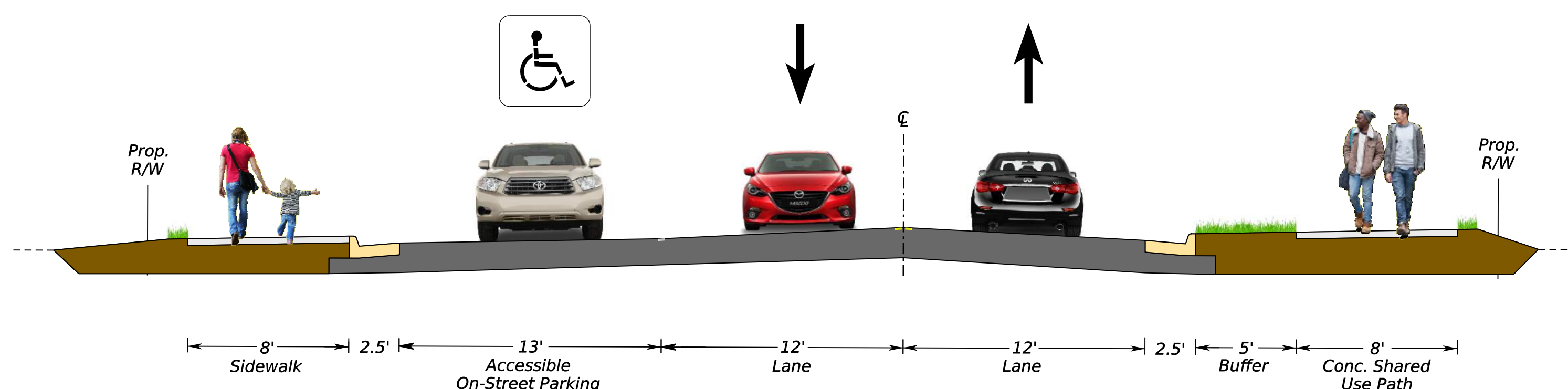
PROPOSED TYPICAL SECTION B-B
