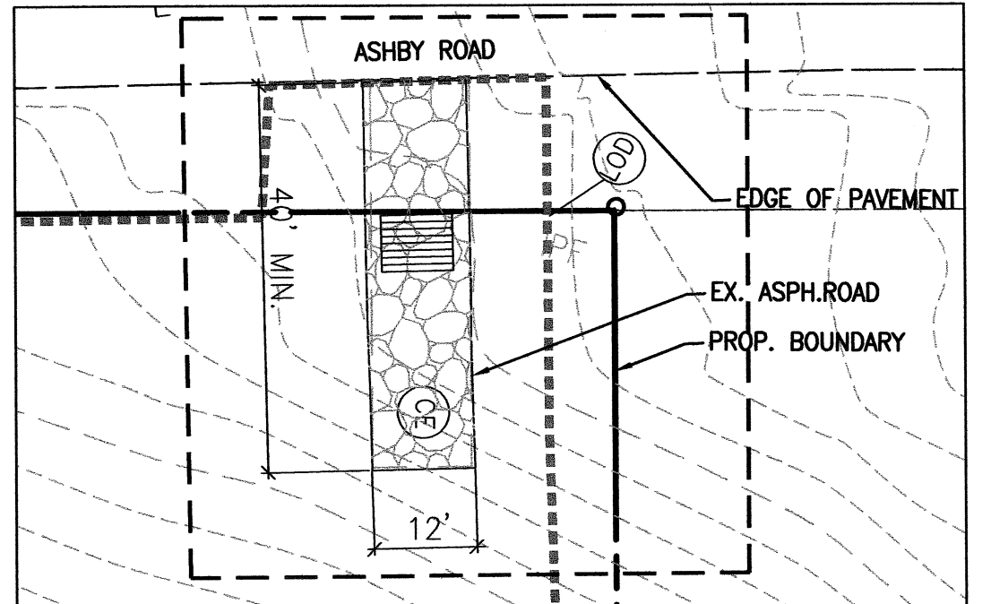
CONSTRUCTION ENTRANCE SCALE: 1" = 20'
