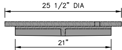
COVER SECTION B-B
