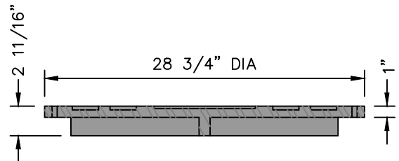
COVER SECTION B-B
