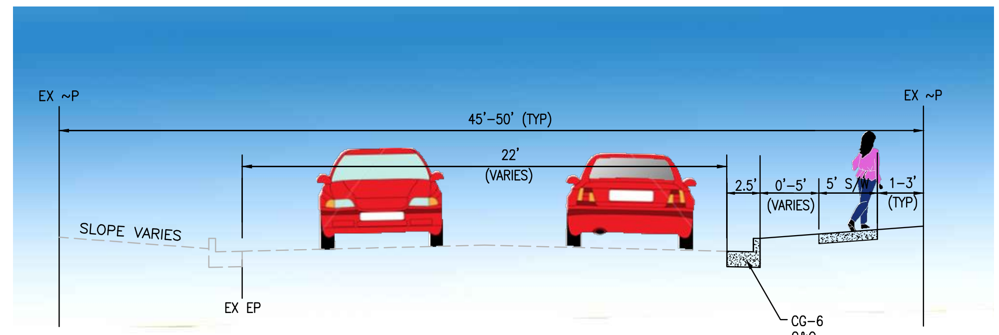
BURKE STATION ROAD TYPICAL STREET SECTION-IMPROVED CONDITION (NOT TO SCALE)
