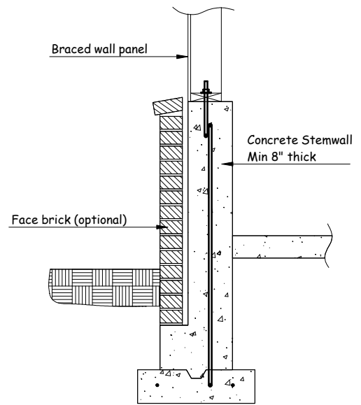
Typical Stemwall Section
