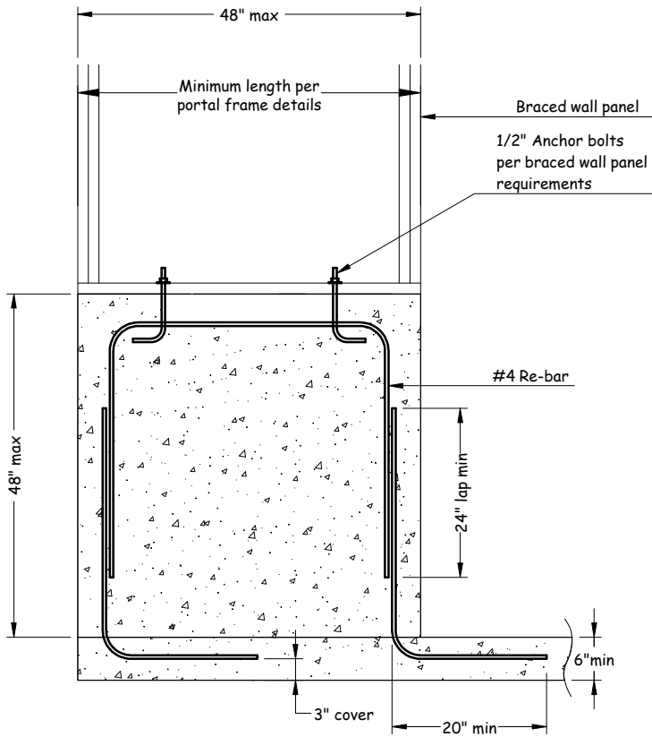
Tall Stemwall Reinforcement
