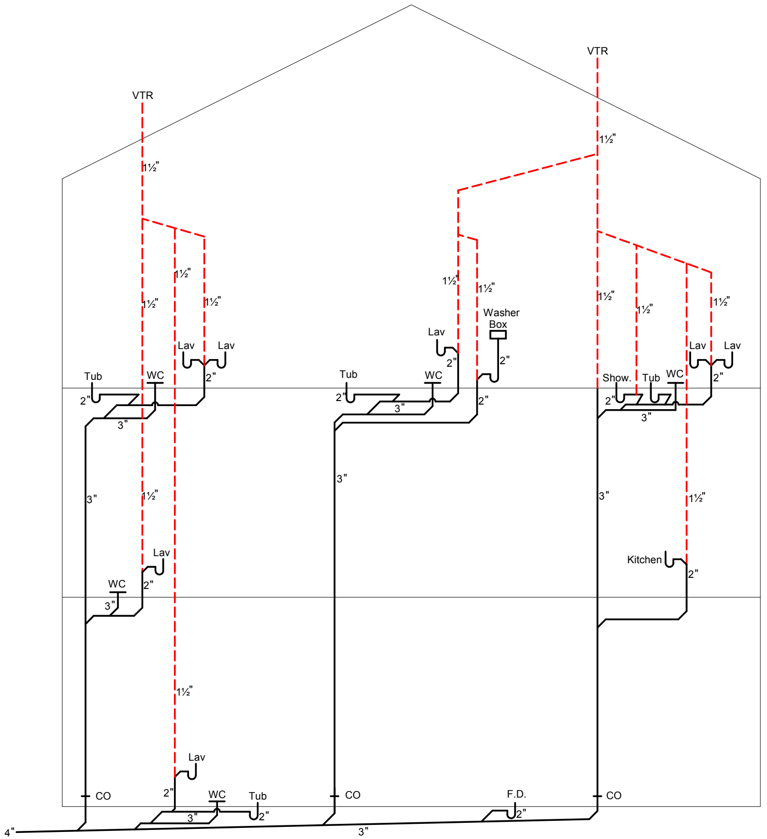
Typical DWV for Single Family House
